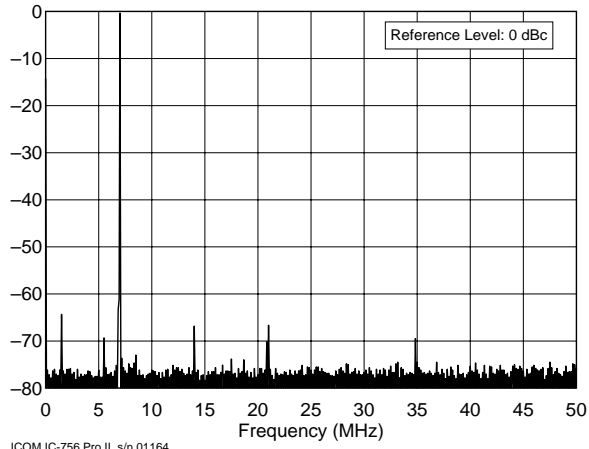
ICOM IC-756 Pro II, s/n 01164 7.0 MHz Band, Spectral Purity, 100 W F:\SHARED\PROD_REV\TESTS\IC756P2\756P2S40.TXT
