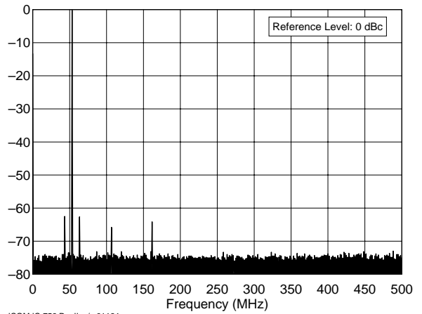
ICOM IC-756 Pro II, s/n 01164 50.0 MHz Band, Spectral Purity, 100 W F:\SHARED\PROD_REV\TESTS\IC756P2\756P2S8M.TXT
