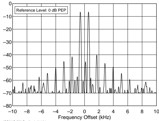
ICOM IC-756 Pro II, s/n 01164 1.850 MHz, Transmit IMD, 100 W F:\SHARED\PROD_REV\TESTS\IC756P2\756P21LO.TXT
