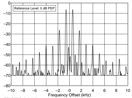
ICOM IC-756 Pro II, s/n 01164 50.200 MHz, Transmit IMD, 100 W F:\SHARED\PROD_REV\TESTS\IC756P2\756P216M.TXT
