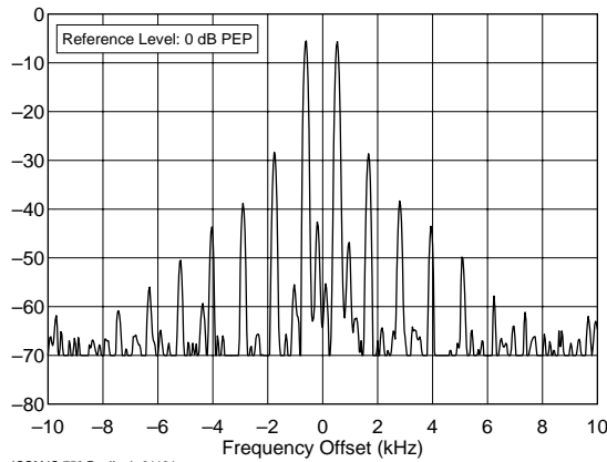
ICOM IC-756 Pro II, s/n 01164 28.350 MHz, Transmit IMD, 100 W F:\SHARED\PROD_REV\TESTS\IC756P2\756P2110.TXT
