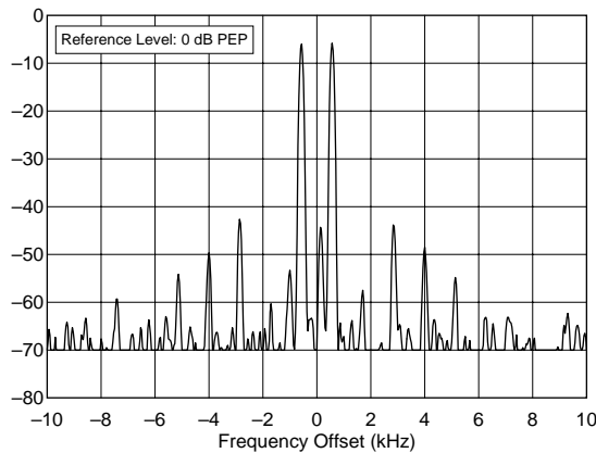
ICOM IC-756 Pro II, s/n 01164 3.900 MHz, Transmit IMD, 100 W F:\SHARED\PROD_REV\TESTS\IC756P2\756P2180.TXT
